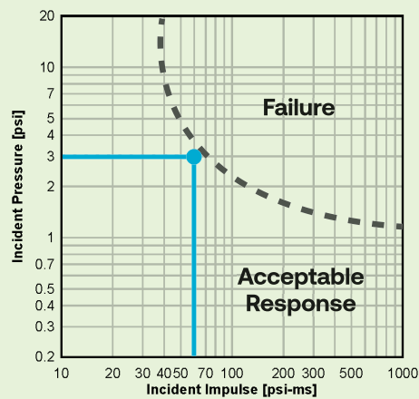
Figure 1. Acceptable Region (Shown in Blue) in P-i Space
