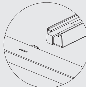
3. Detail of „Snap in system“ of substructure
