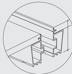
1. Tongue and groove floor cassettes
