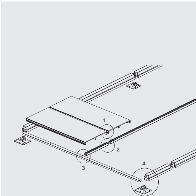
System cassette flooring with integrated cable channel and variable cable exit positioning
