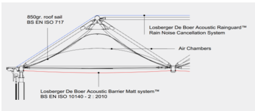
Acoustic roof detail
