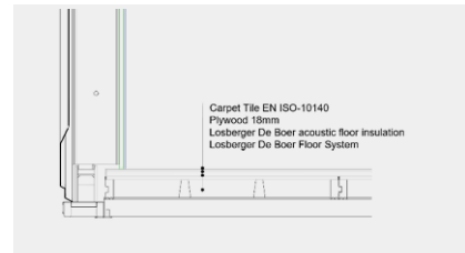
Acoustic floor detail
