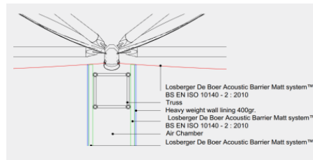
Acoustic wall detail
