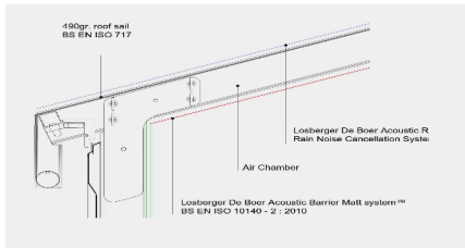
Acoustic roof detail
