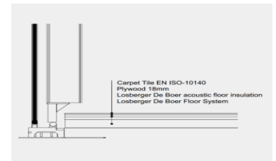
Acoustic floor detail
