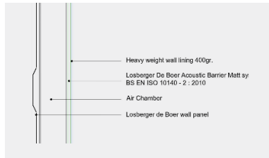
Acoustic wall detail
